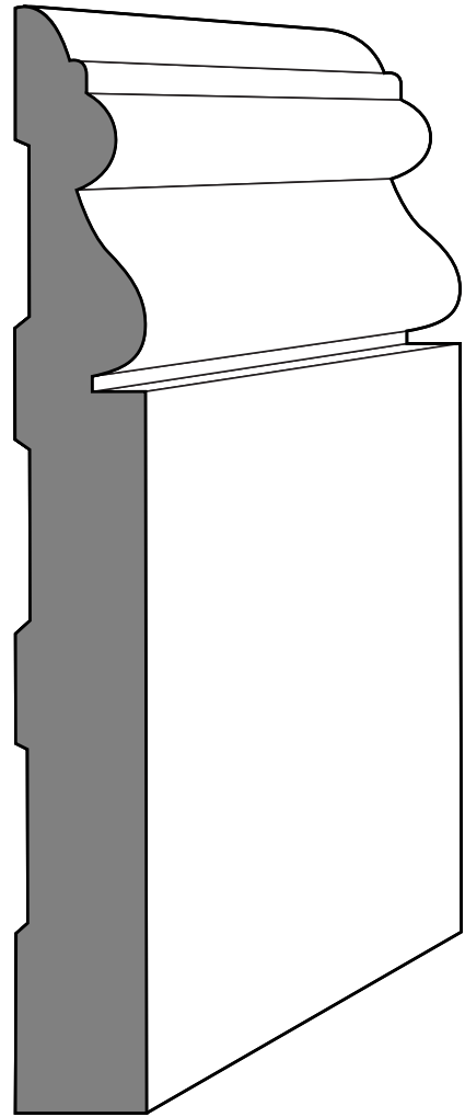
5 1/4" Lower
